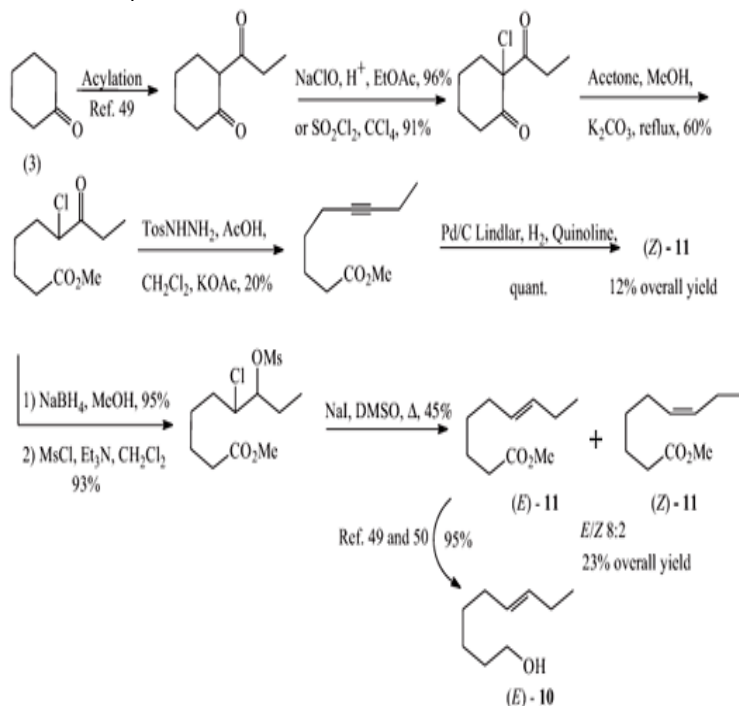
Scheme 10.
